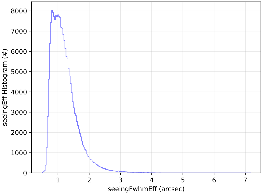
start_date_do-360v3.4_10yrs WFD g band: seeingEff Histogram
