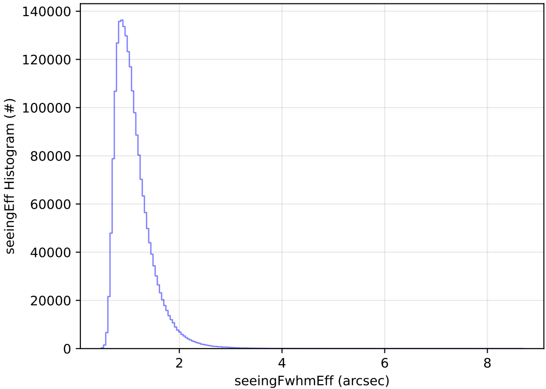
start_date_do-360v3.4_10yrs WFD all bands: seeingEff Histogram
