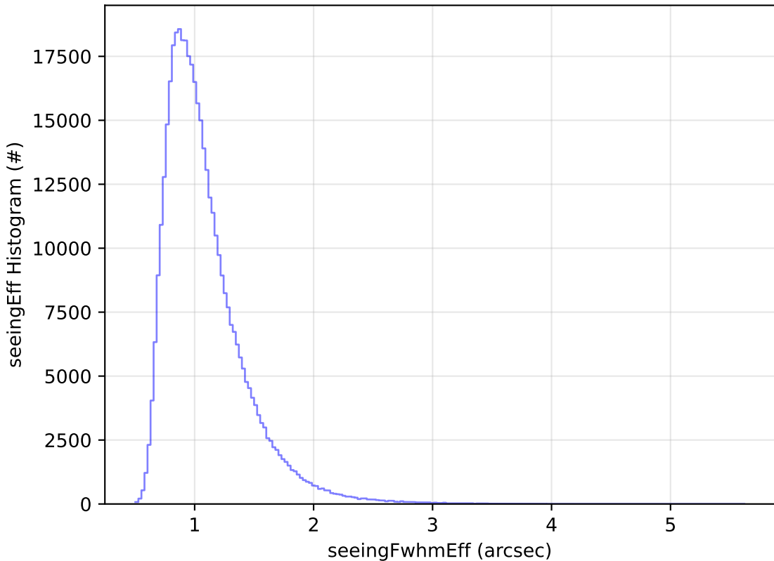
start_date_do-360v3.4_10yrs All sky z band: seeingEff Histogram
