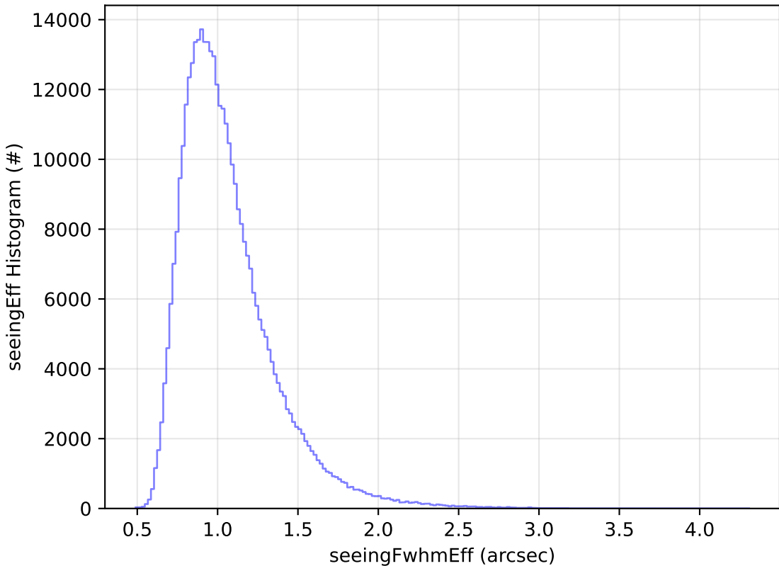
start_date_do-360v3.4_10yrs All sky y band: seeingEff Histogram
