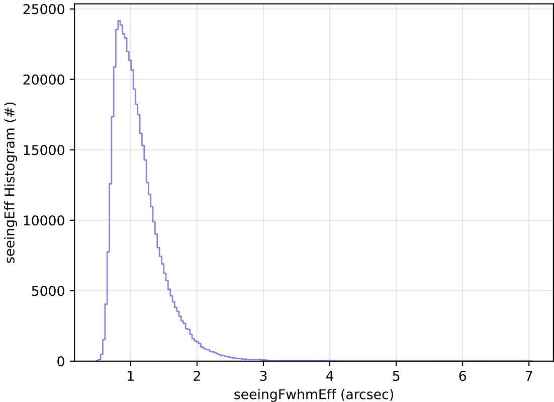
start_date_do-360v3.4_10yrs All sky r band: seeingEff Histogram
