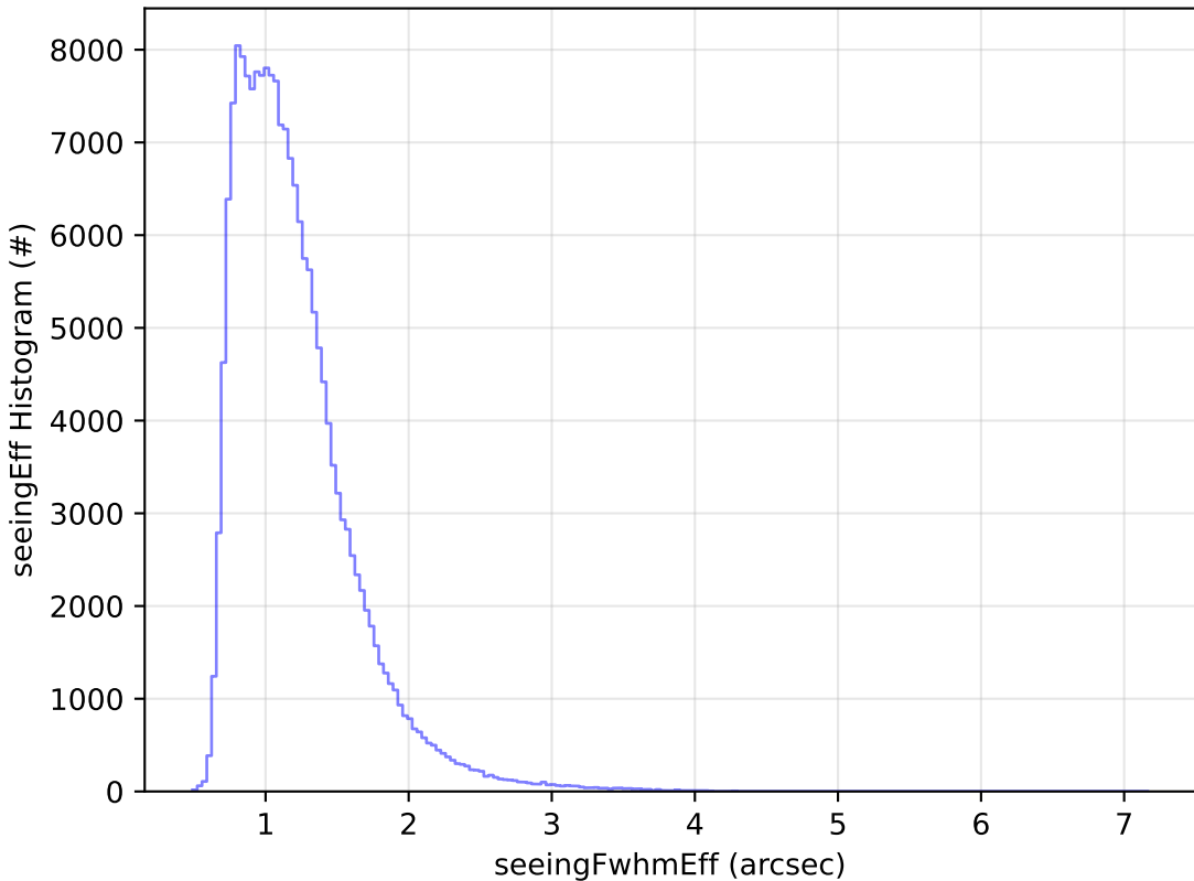
start_date_do-360v3.4_10yrs All sky g band: seeingEff Histogram
