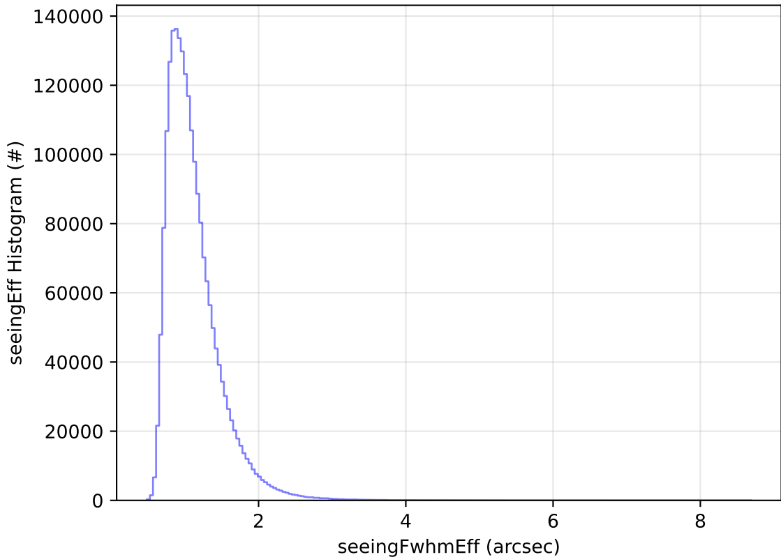
start_date_do-360v3.4_10yrs All sky all bands: seeingEff Histogram
