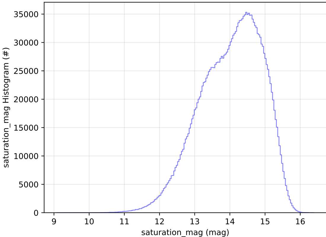
start_date_do-360v3.4_10yrs WFD all bands: saturation_mag Histogram
