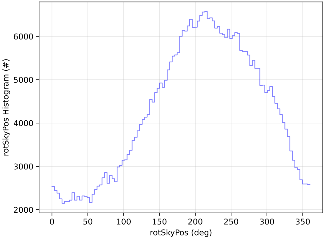
start_date_do-360v3.4_10yrs WFD z band: rotSkyPos Histogram
