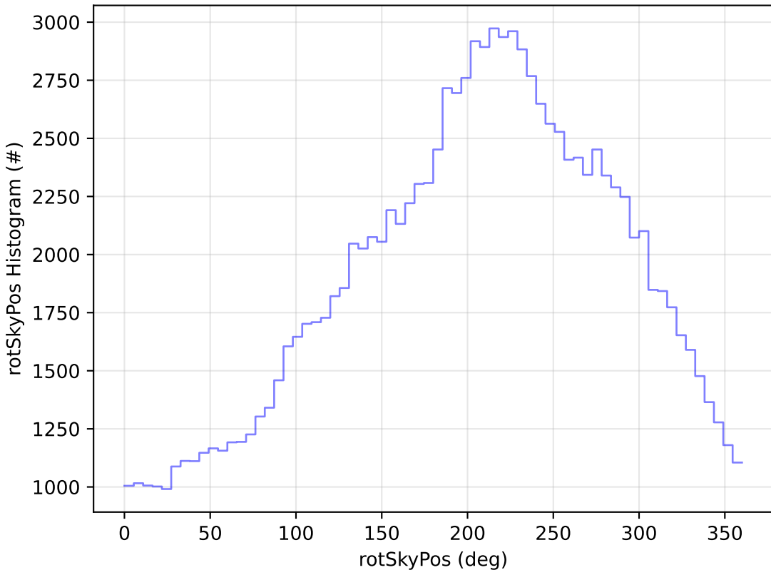
start_date_do-360v3.4_10yrs WFD u band: rotSkyPos Histogram
