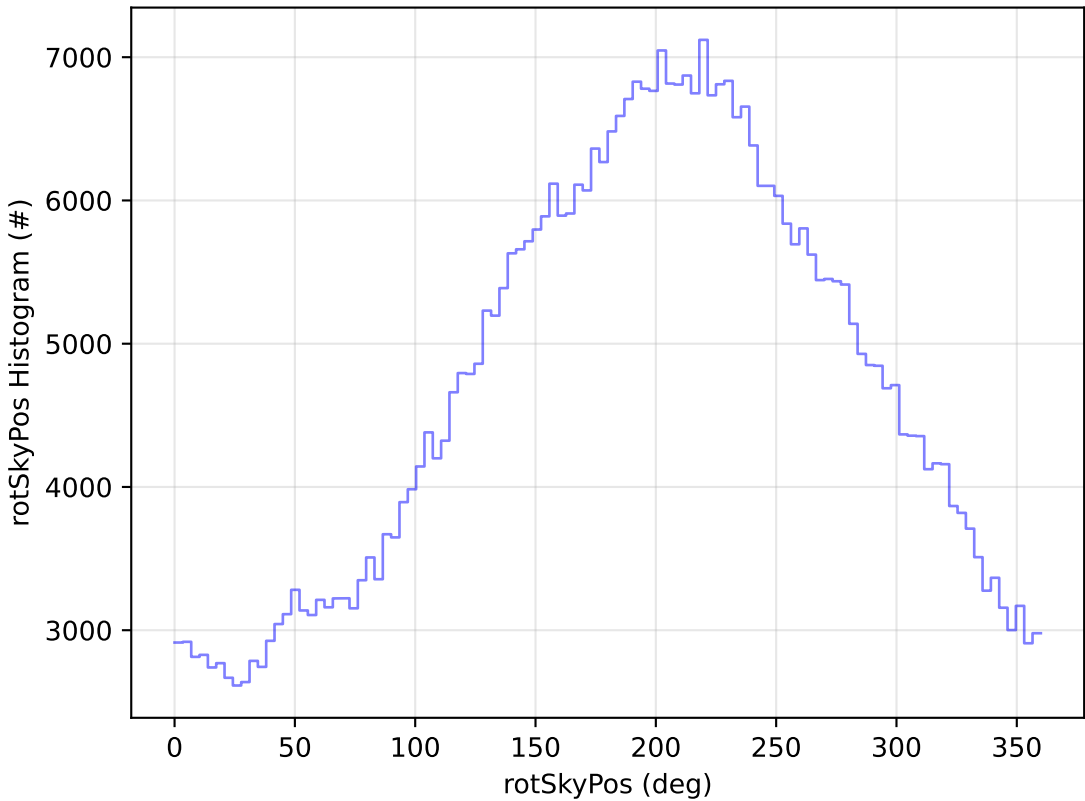
start_date_do-360v3.4_10yrs WFD r band: rotSkyPos Histogram
