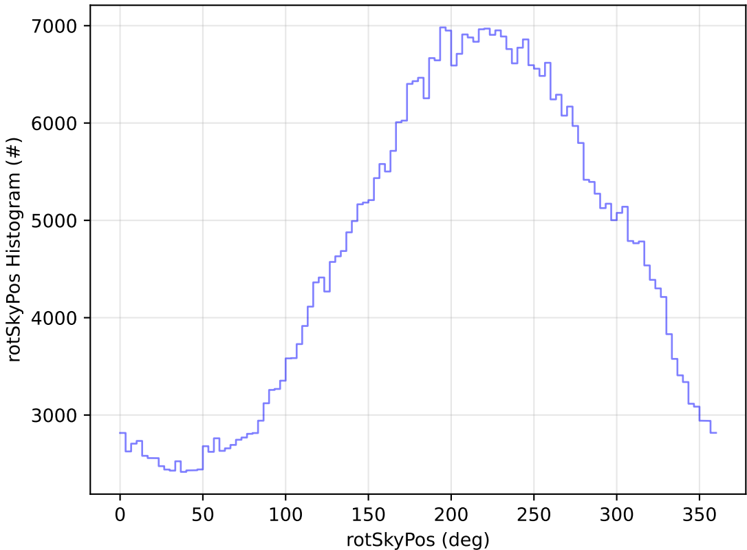
start_date_do-360v3.4_10yrs WFD i band: rotSkyPos Histogram
