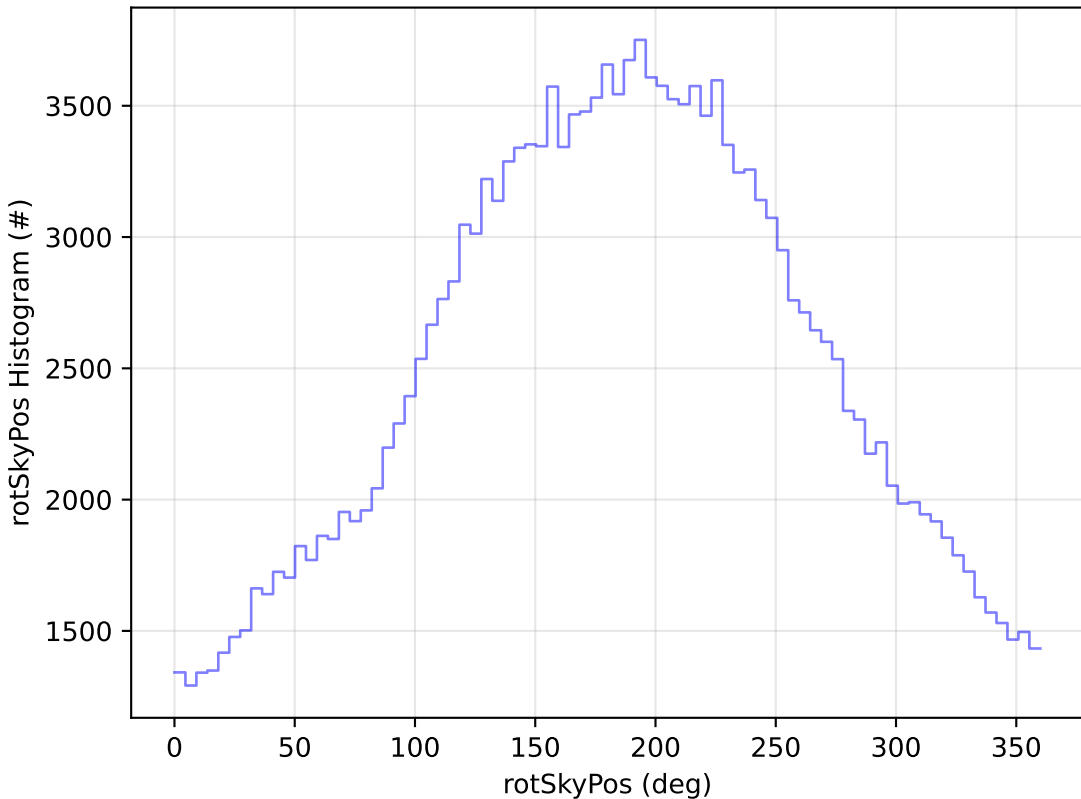
start_date_do-360v3.4_10yrs WFD g band: rotSkyPos Histogram
