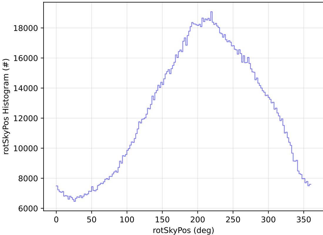
start_date_do-360v3.4_10yrs WFD all bands: rotSkyPos Histogram
