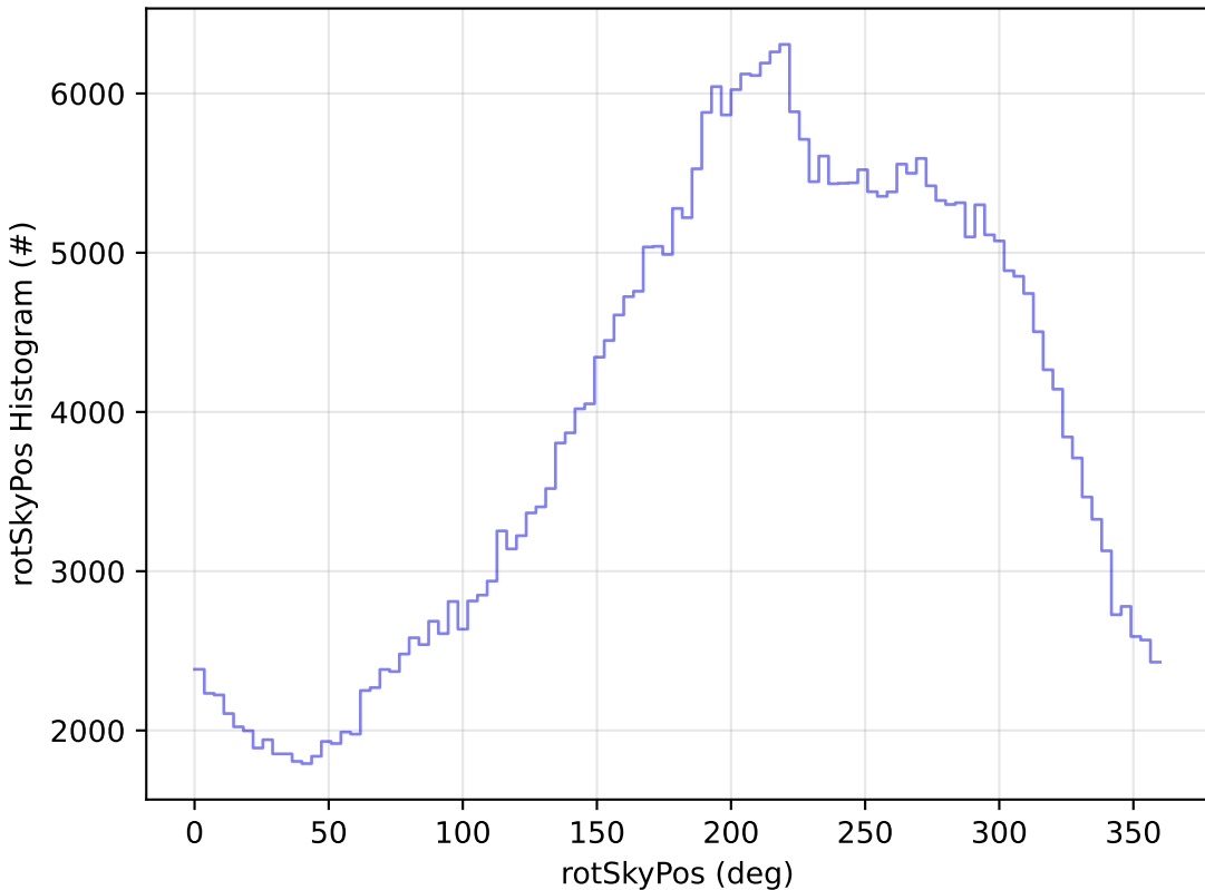
start_date_do-360v3.4_10yrs All sky y band: rotSkyPos Histogram
