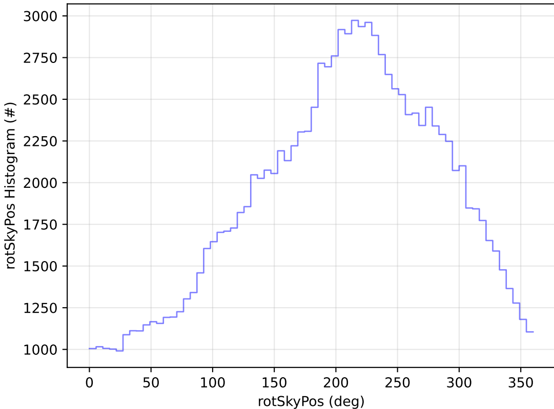
start_date_do-360v3.4_10yrs All sky u band: rotSkyPos Histogram
