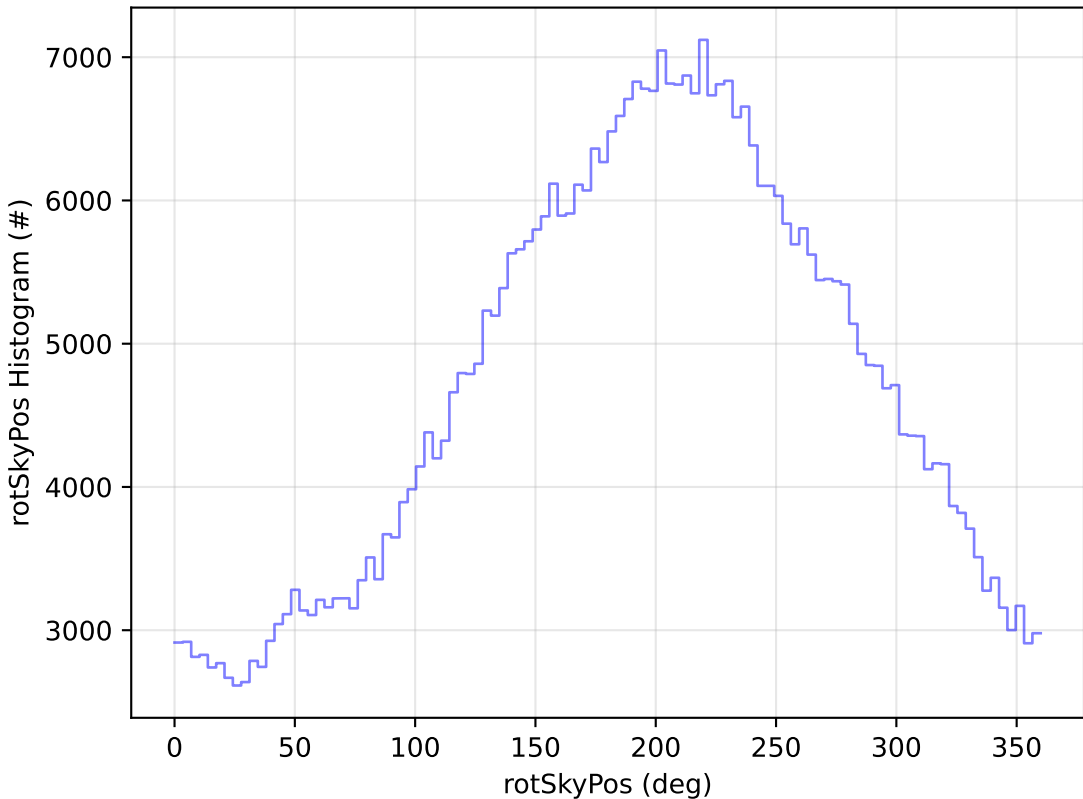
start_date_do-360v3.4_10yrs All sky r band: rotSkyPos Histogram
