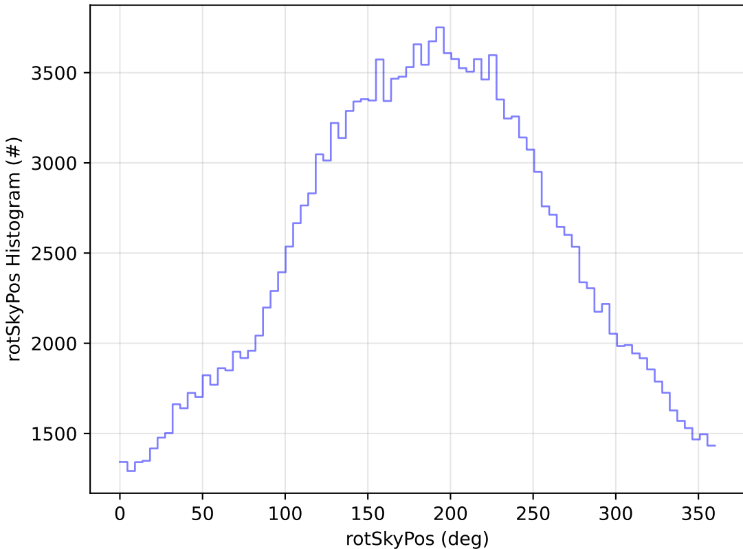
start_date_do-360v3.4_10yrs All sky g band: rotSkyPos Histogram
