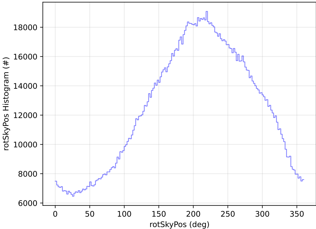
start_date_do-360v3.4_10yrs All sky all bands: rotSkyPos Histogram
