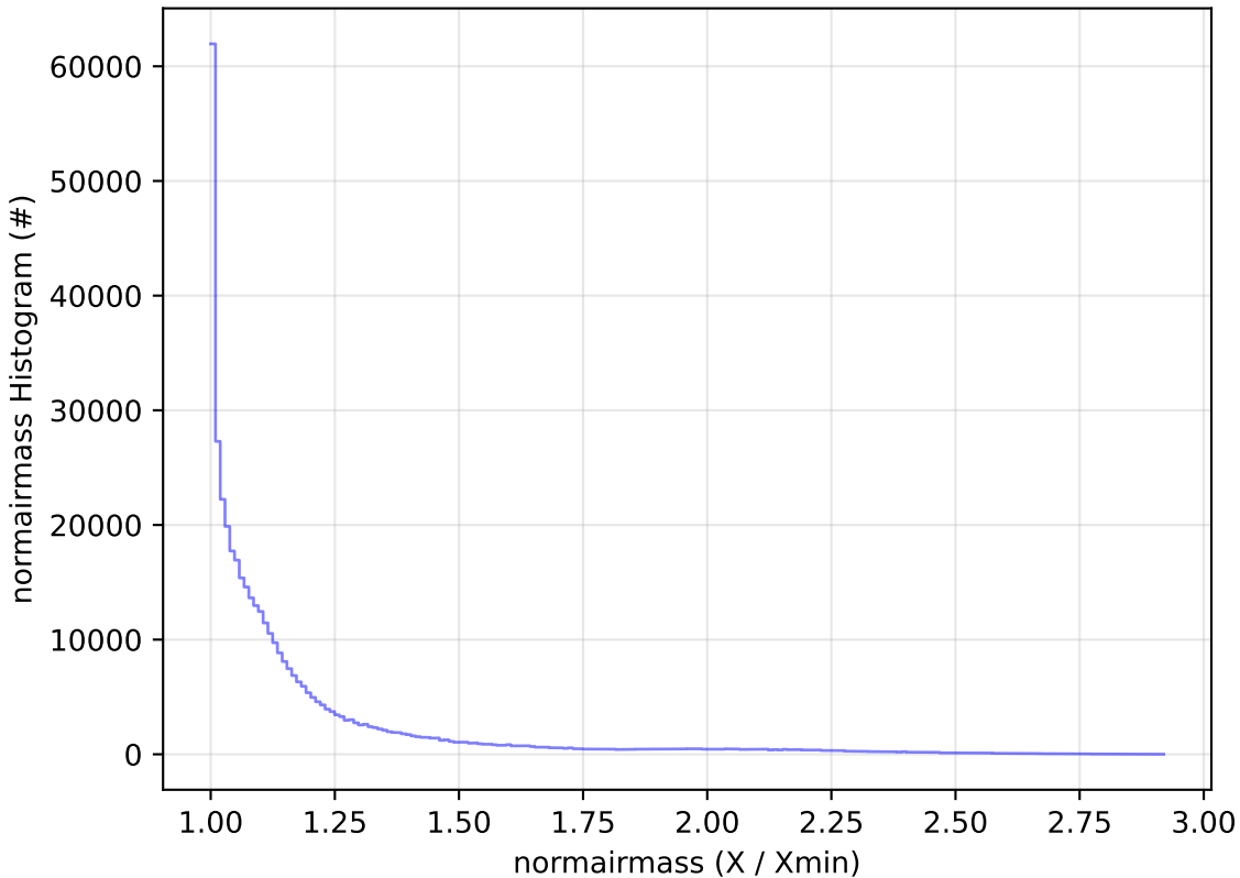
start_date_do-360v3.4_10yrs WFD z band: normairmass Histogram
