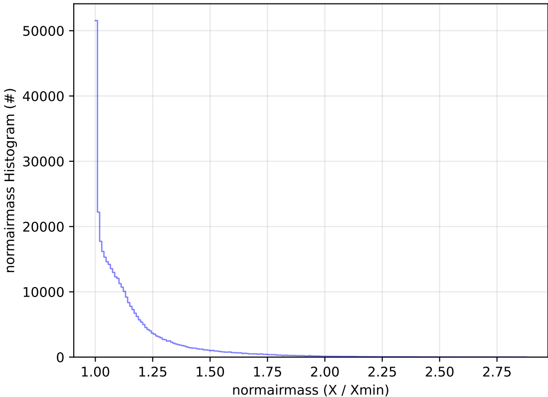
start_date_do-360v3.4_10yrs WFD y band: normairmass Histogram
