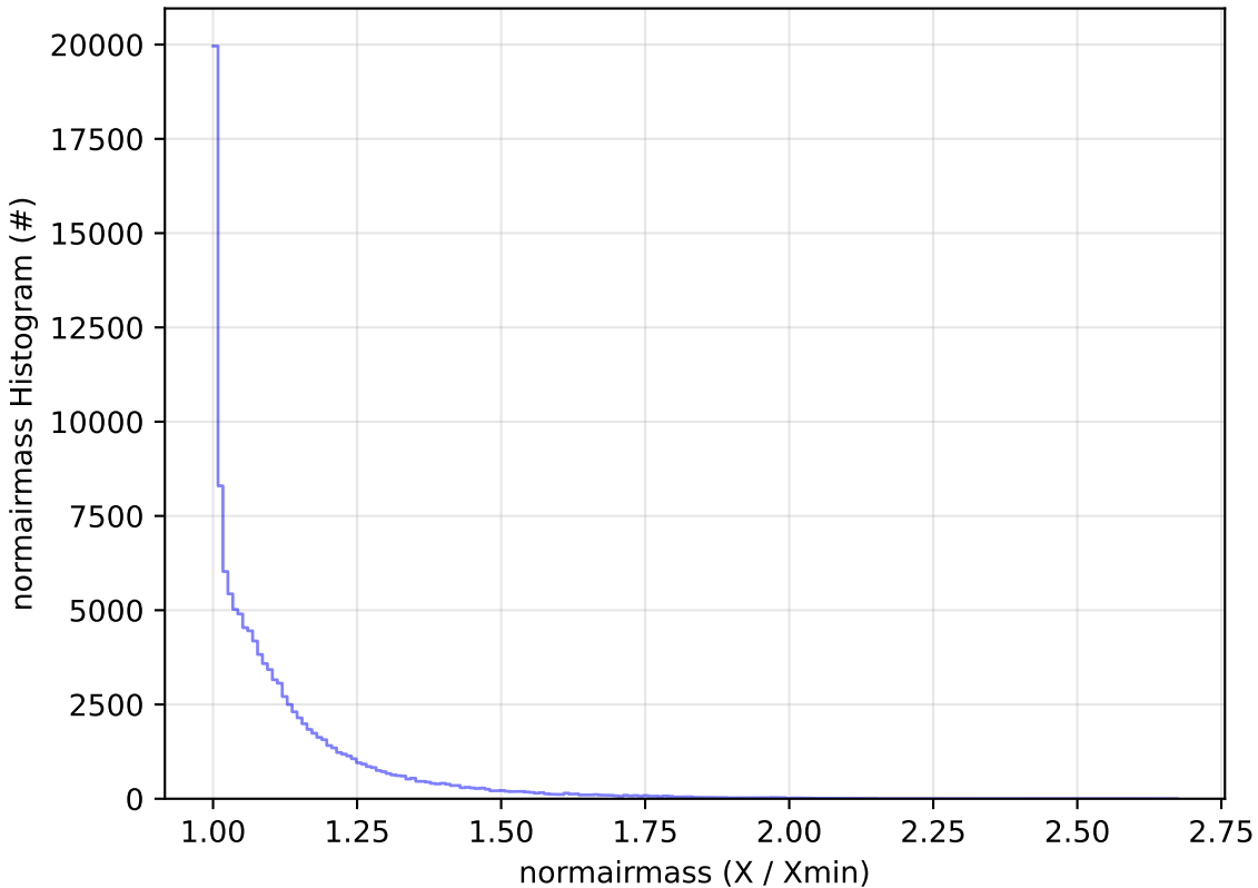
start_date_do-360v3.4_10yrs WFD u band: normairmass Histogram
