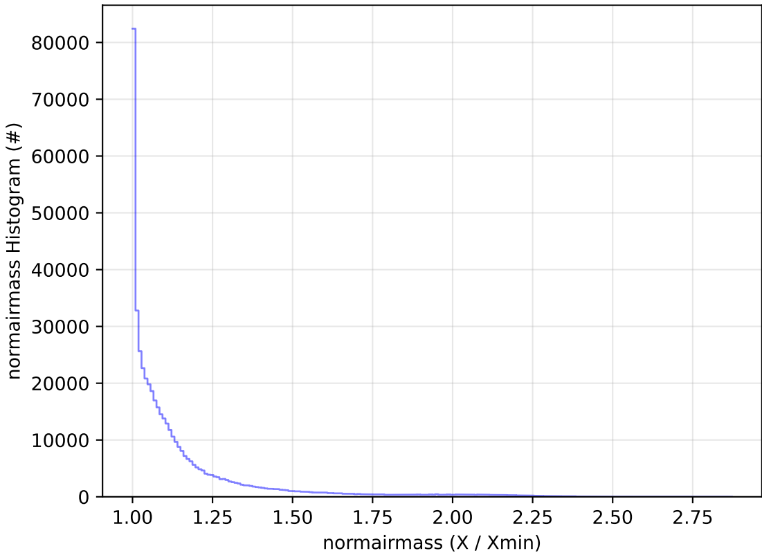
start_date_do-360v3.4_10yrs WFD r band: normairmass Histogram
