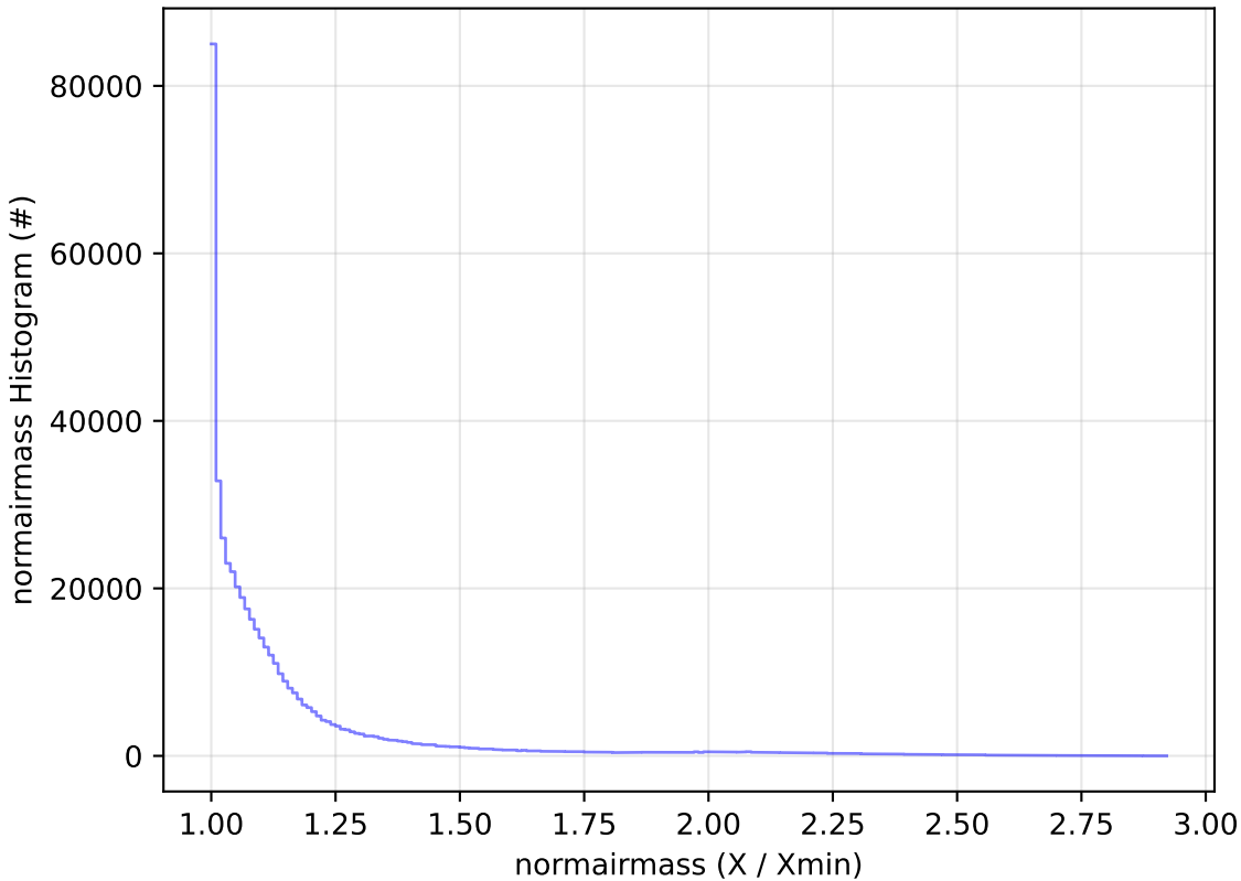
start_date_do-360v3.4_10yrs WFD i band: normairmass Histogram
