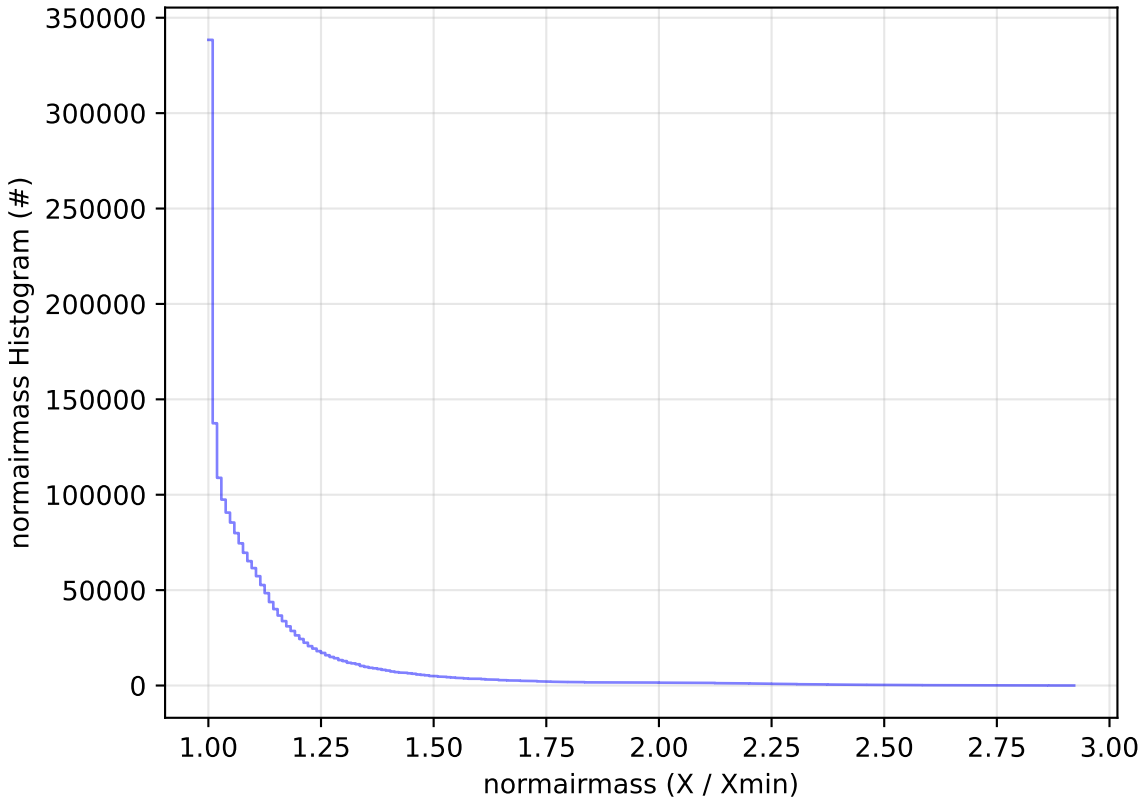
start_date_do-360v3.4_10yrs WFD all bands: normairmass Histogram
