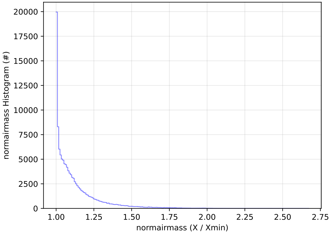
start_date_do-360v3.4_10yrs All sky u band: normairmass Histogram
