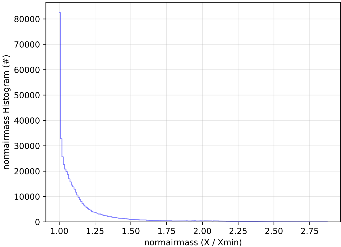
start_date_do-360v3.4_10yrs All sky r band: normairmass Histogram
