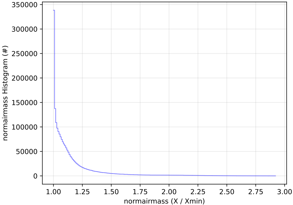
start_date_do-360v3.4_10yrs All sky all bands: normairmass Histogram
