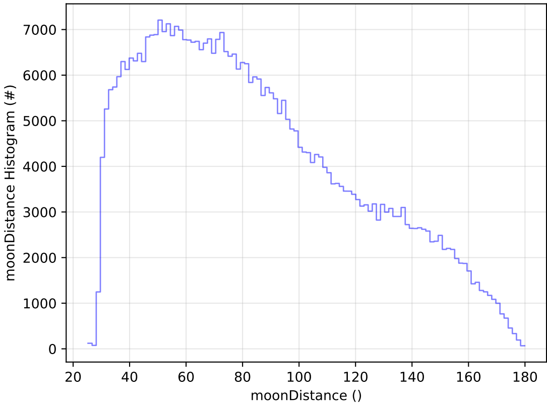
start_date_do-360v3.4_10yrs WFD z band: moonDistance Histogram
