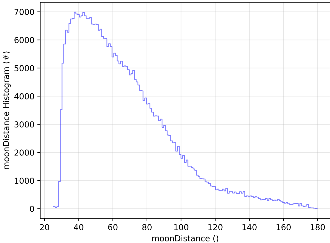
start_date_do-360v3.4_10yrs WFD y band: moonDistance Histogram
