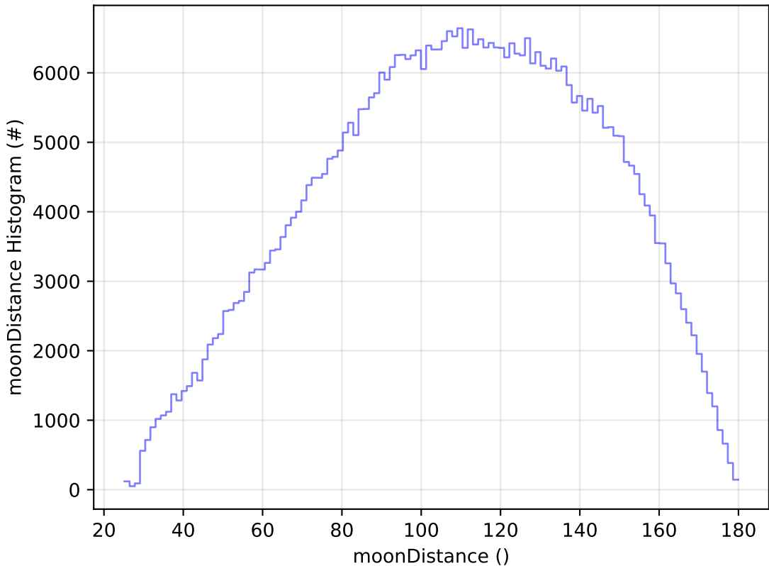
start_date_do-360v3.4_10yrs WFD r band: moonDistance Histogram
