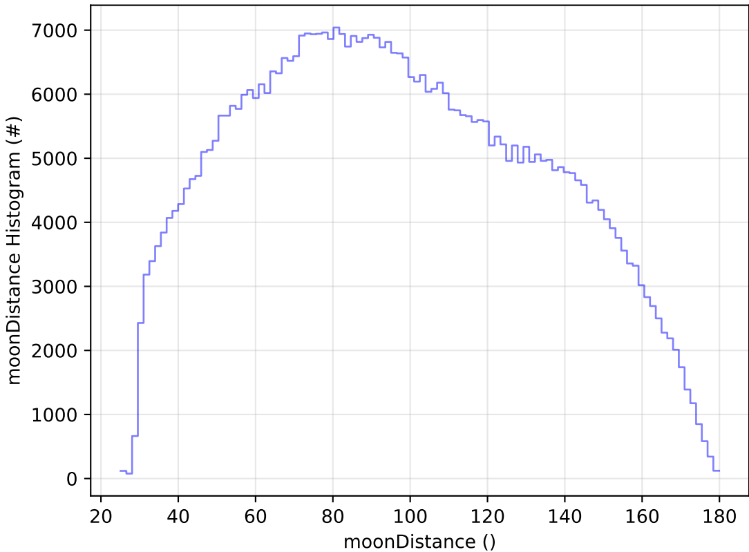
start_date_do-360v3.4_10yrs WFD i band: moonDistance Histogram
