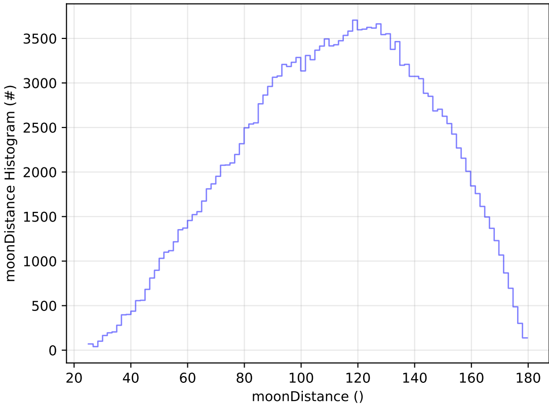
start_date_do-360v3.4_10yrs WFD g band: moonDistance Histogram
