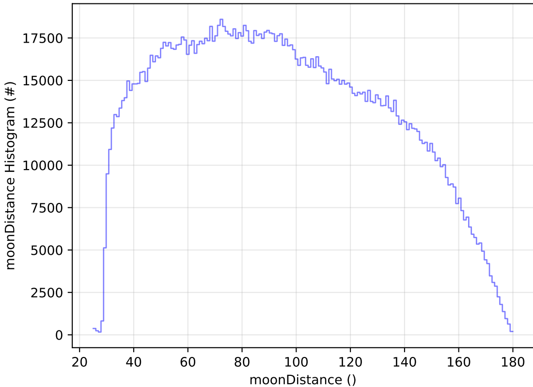
start_date_do-360v3.4_10yrs WFD all bands: moonDistance Histogram
