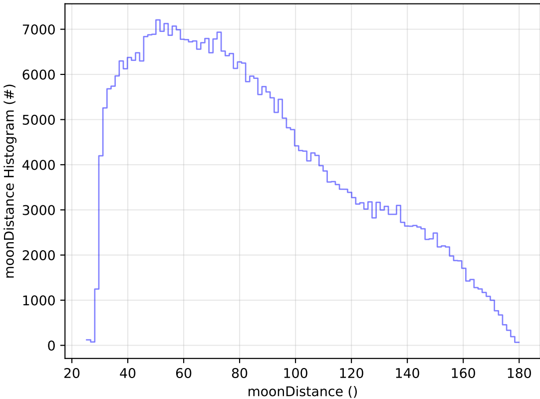
start_date_do-360v3.4_10yrs All sky z band: moonDistance Histogram
