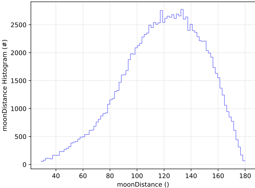
start_date_do-360v3.4_10yrs All sky u band: moonDistance Histogram
