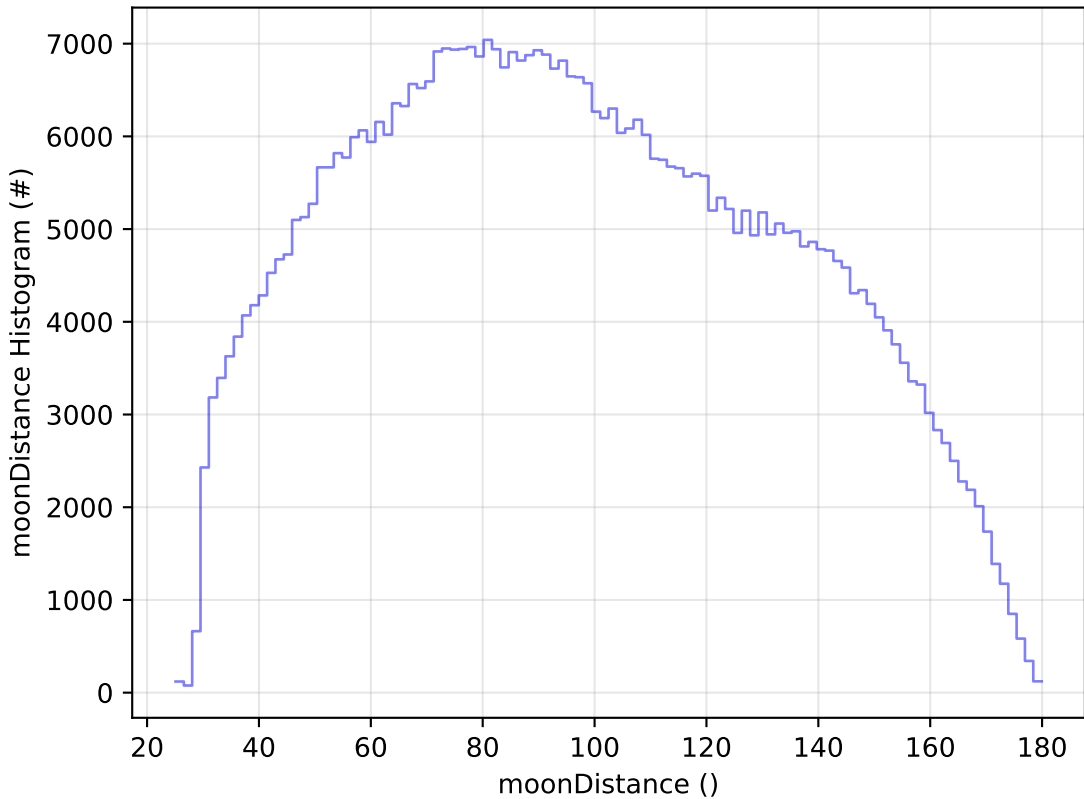
start_date_do-360v3.4_10yrs All sky i band: moonDistance Histogram
