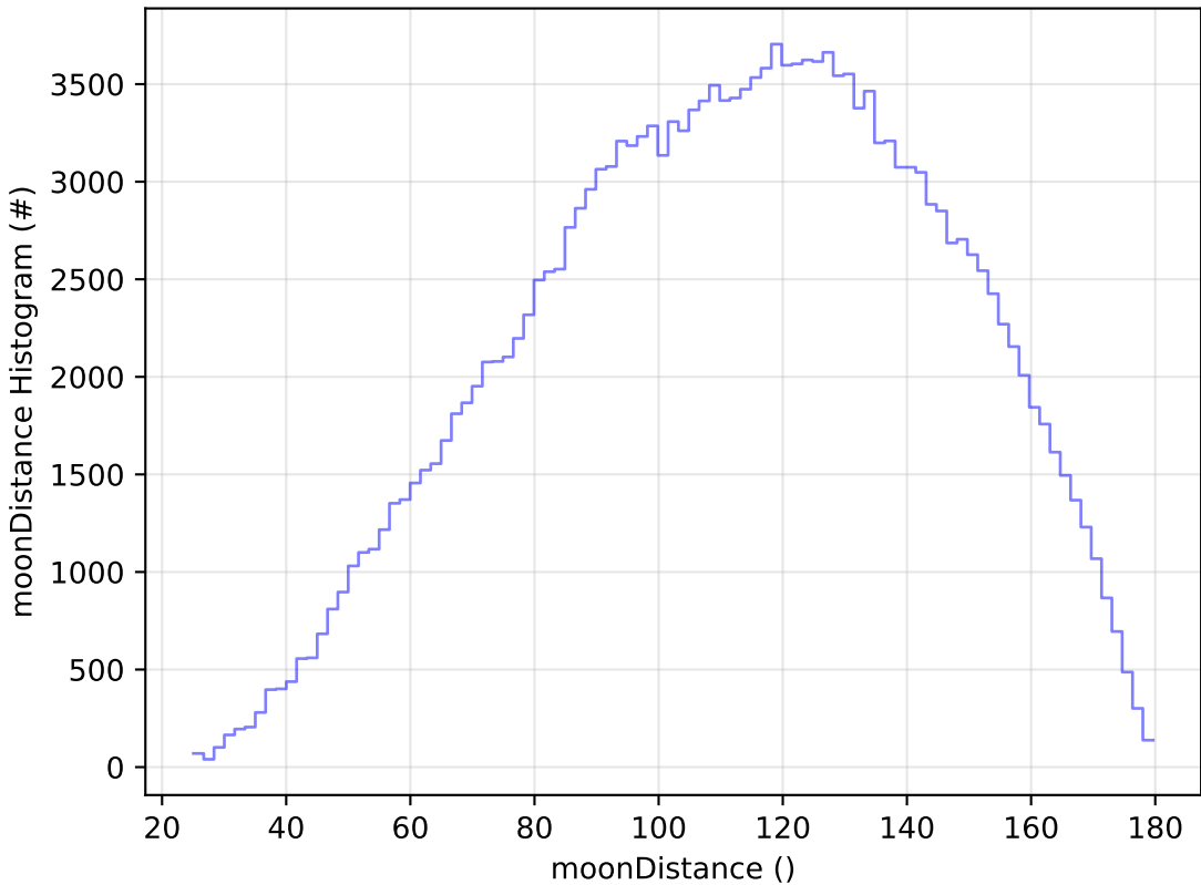
start_date_do-360v3.4_10yrs All sky g band: moonDistance Histogram
