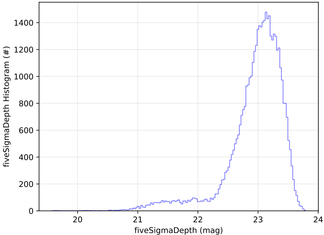
start_date_do-360v3.4_10yrs Yr 1 z band: fiveSigmaDepth Histogram
