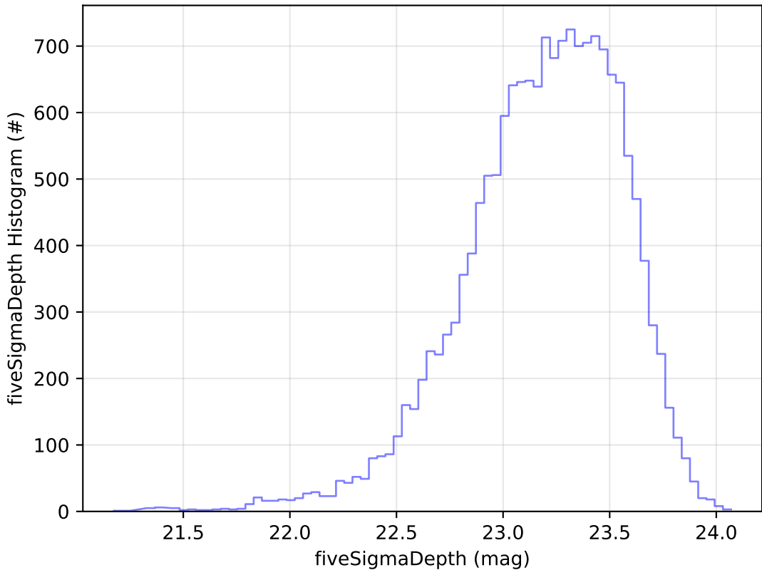
start_date_do-360v3.4_10yrs Yr 1 u band: fiveSigmaDepth Histogram
