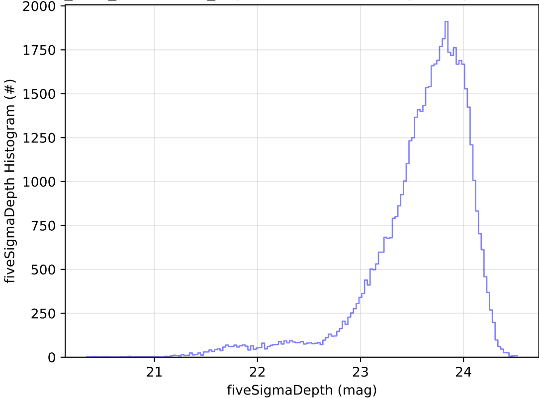
start_date_do-360v3.4_10yrs Yr 1 i band: fiveSigmaDepth Histogram
