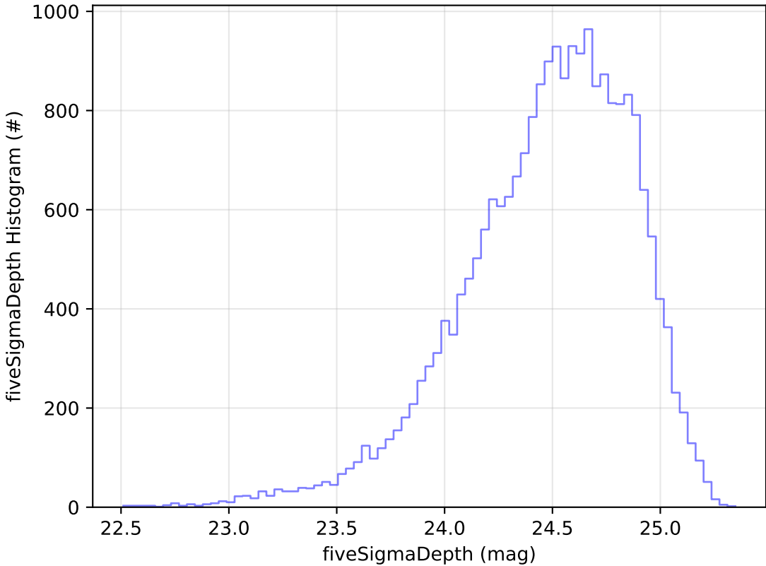
start_date_do-360v3.4_10yrs Yr 1 g band: fiveSigmaDepth Histogram
