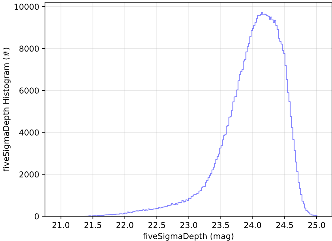
start_date_do-360v3.4_10yrs WFD r band: fiveSigmaDepth Histogram
