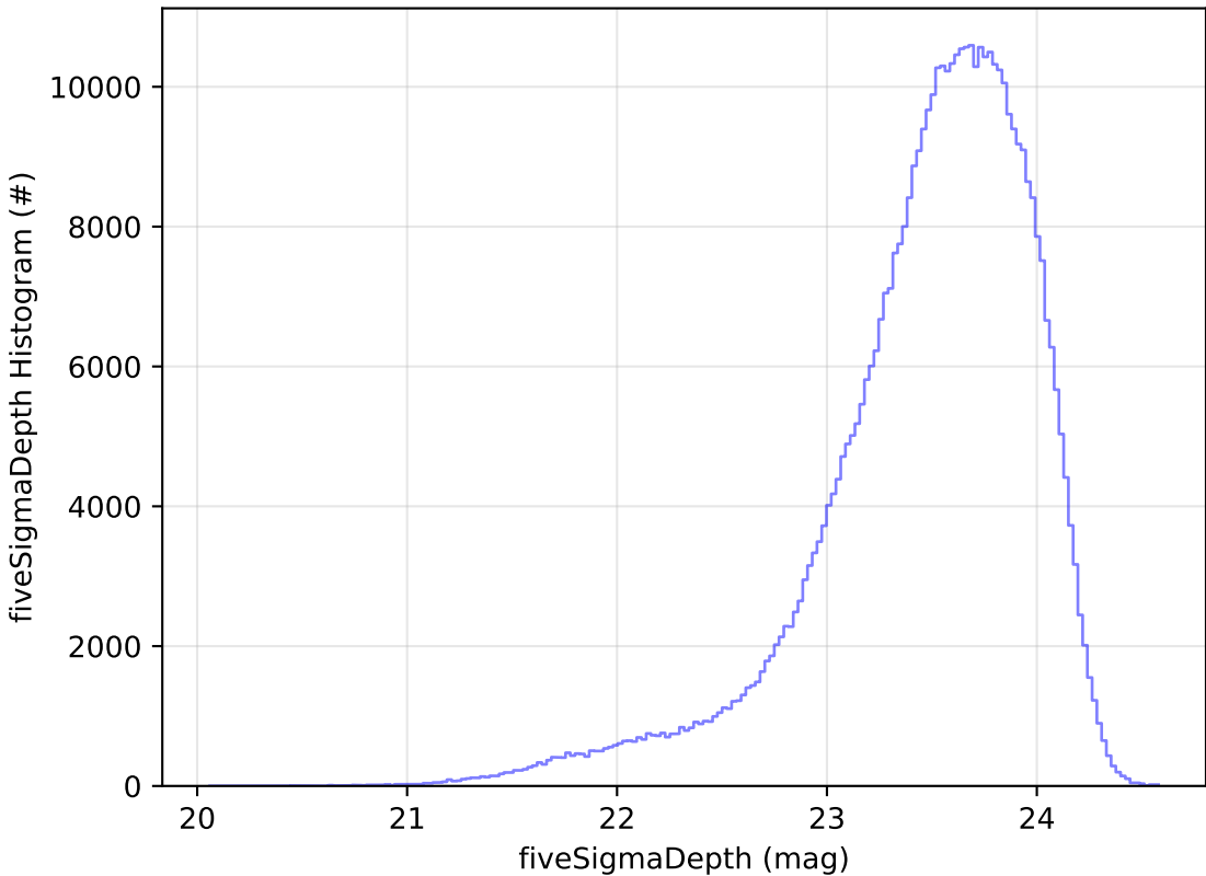
start_date_do-360v3.4_10yrs WFD i band: fiveSigmaDepth Histogram
