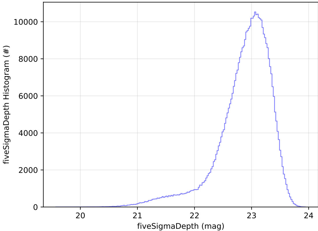
start_date_do-360v3.4_10yrs All sky z band: fiveSigmaDepth Histogram
