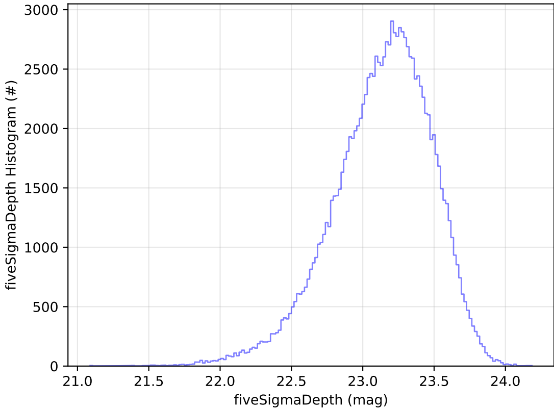
start_date_do-360v3.4_10yrs All sky u band: fiveSigmaDepth Histogram
