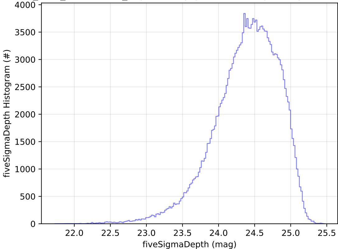
start_date_do-360v3.4_10yrs All sky g band: fiveSigmaDepth Histogram
