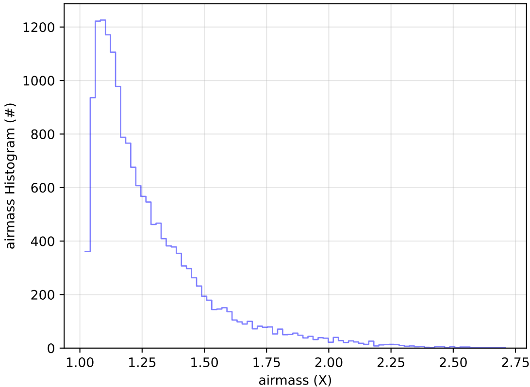
start_date_do-360v3.4_10yrs Yr 1 u band: airmass Histogram
