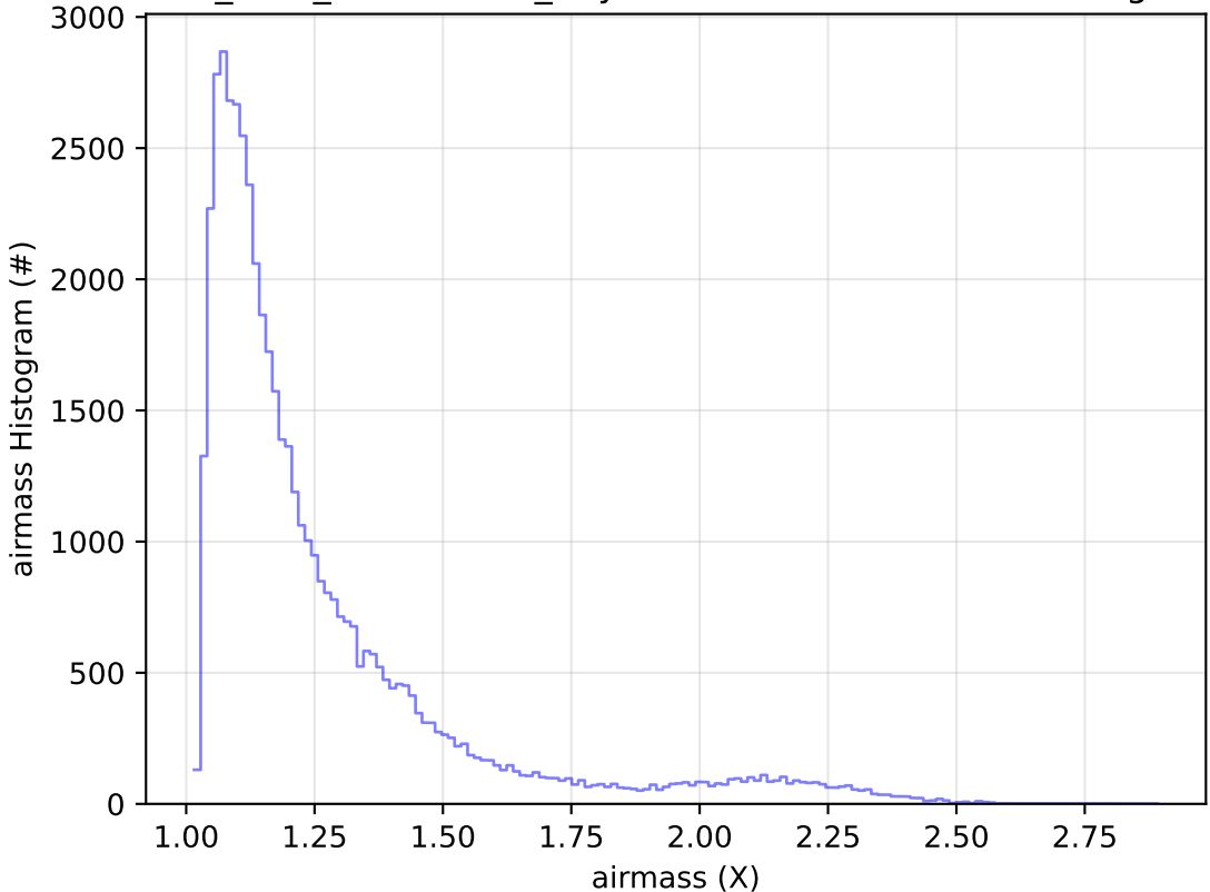
start_date_do-360v3.4_10yrs Yr 1 r band: airmass Histogram
