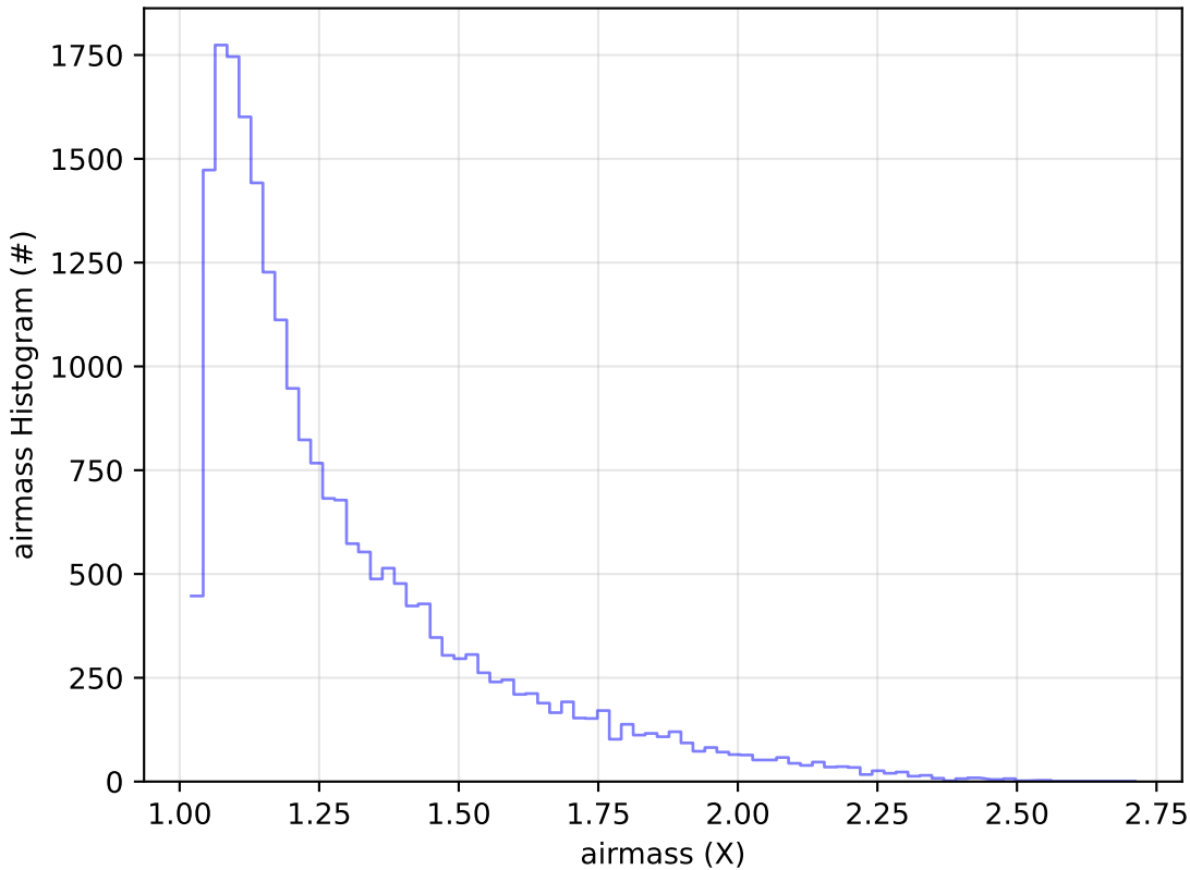
start_date_do-360v3.4_10yrs Yr 1 g band: airmass Histogram
